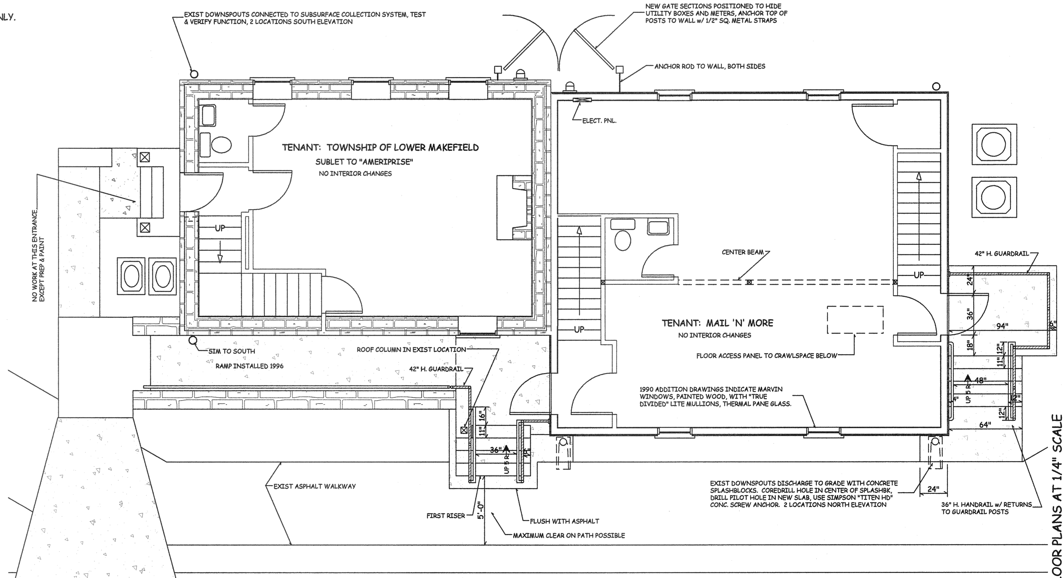
2 2 GROUND (FIRST) FLOOR PLAN SCALE: 1/4" = 1'-0"
